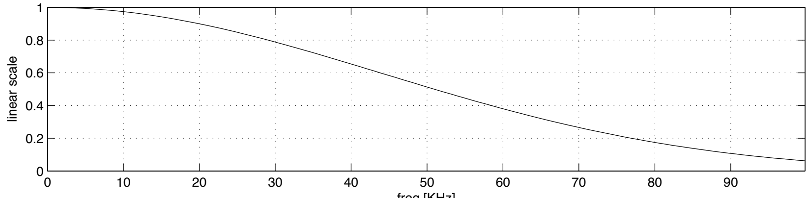
DDF power response, 0 .. HDF output rate
