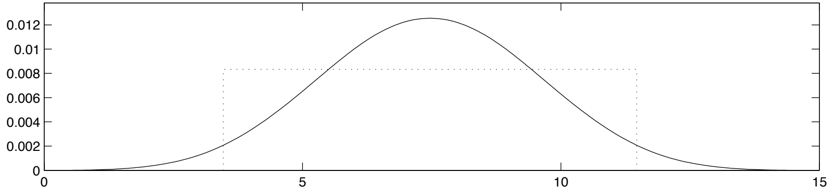
DDF power response, 0 .. FIR output rate
