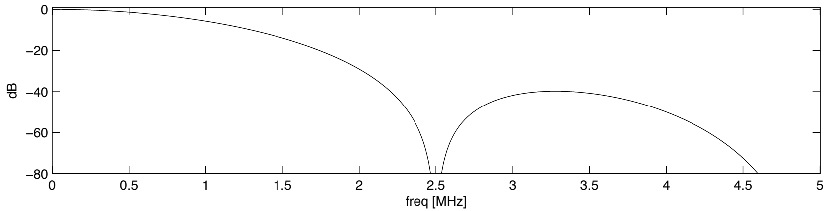
DDF power response, 0 .. HDF output rate
