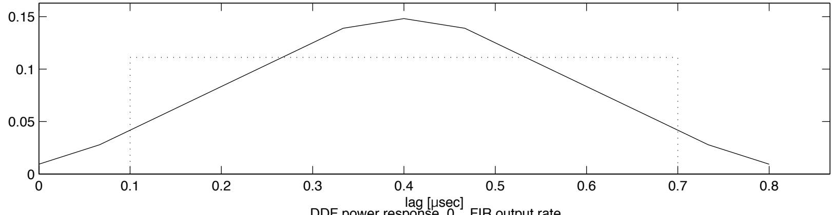
DDF power response, 0 .. FIR output rate
