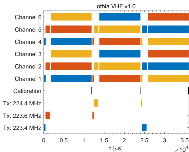
Illustration of timing for transmission and the receiver channels for othia VHF.
