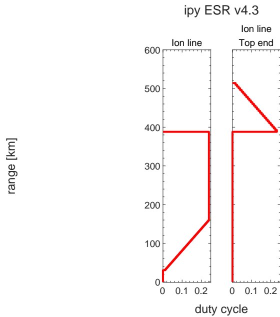
Range coverage for the most relevant data obtained by ipy ESR.
