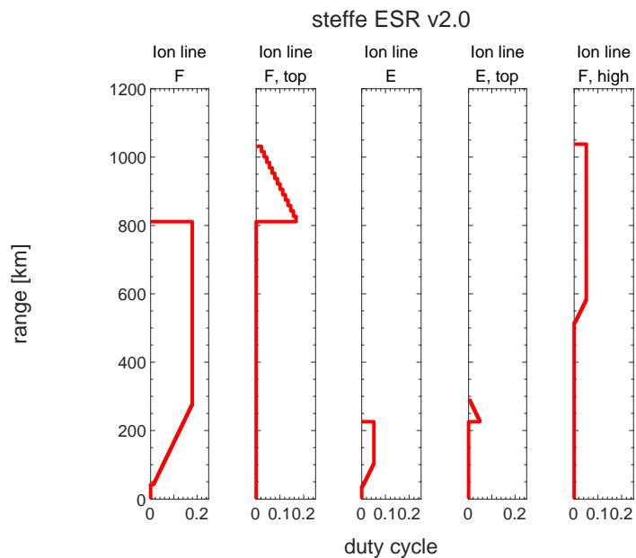
Range coverage for the most relevant data obtained by steffe ESR.
