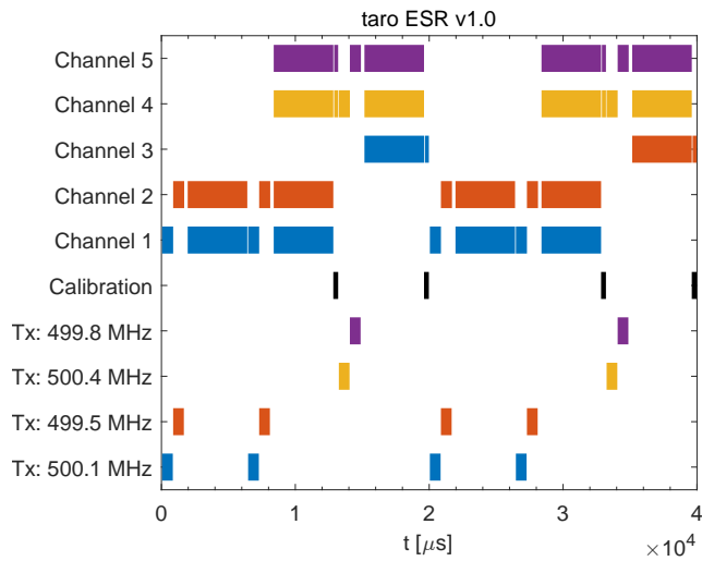
Illustration of timing for transmission and the receiver channels for taro ESR.
