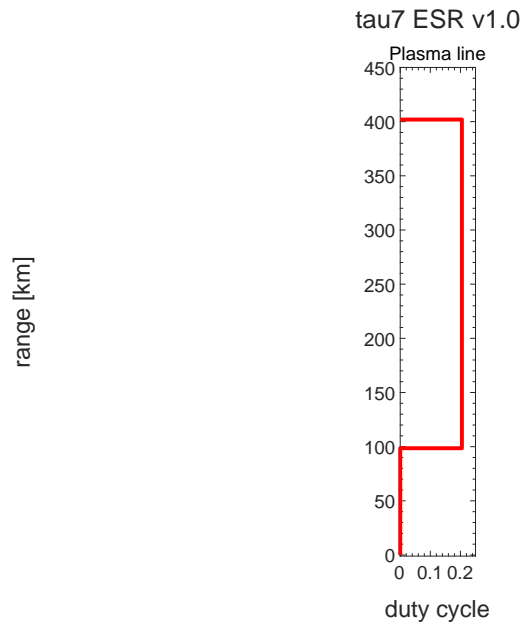
Range coverage for the most relevant data obtained by tau7 ESR plasma line receiver.
