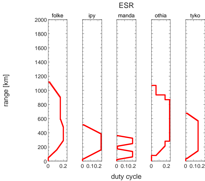
Figure 4: Overview of the ranges covered at the EISCAT ESR radar by the experiments used in the common programmes.
