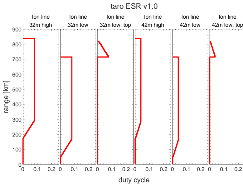
Range coverage for the most relevant data obtained by taro ESR.
