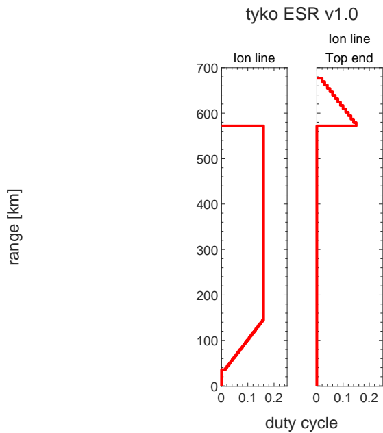
Range coverage for the most relevant data obtained by tyko ESR.
