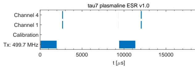
Illustration of timing for transmission and the receiver channels for tau7 ESR plasma line receiver.
